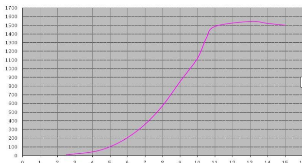
EN-1.5KW-L wind turbine power curve
