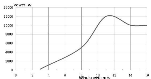
EN-10KW-E wind turbine power curve
