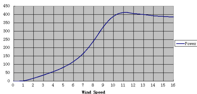
EN-400W-M wind turbine power curve
