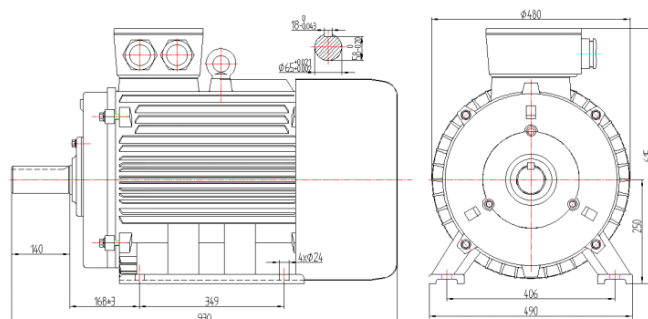
EN-50KW-900R-60Hz-240V Drawing
