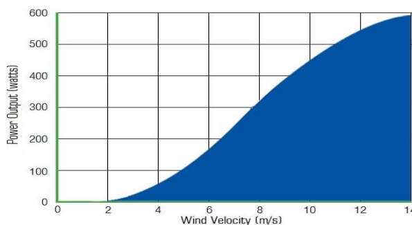
EN-600W-HX wind turbine power curve
